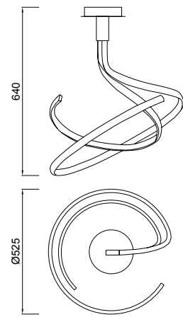
REF.5364 Plafón - Ceiling Lamp
